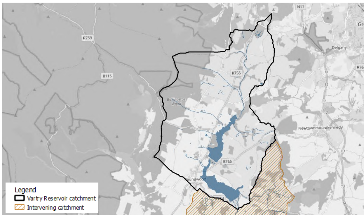
Figure 4-8: Reservoir routing catchment
