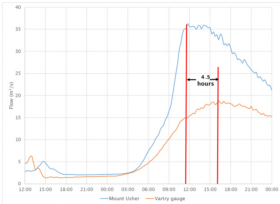
Figure 4-11: Comparison of Vartry and Mount Usher gauge for Jan 30th event
