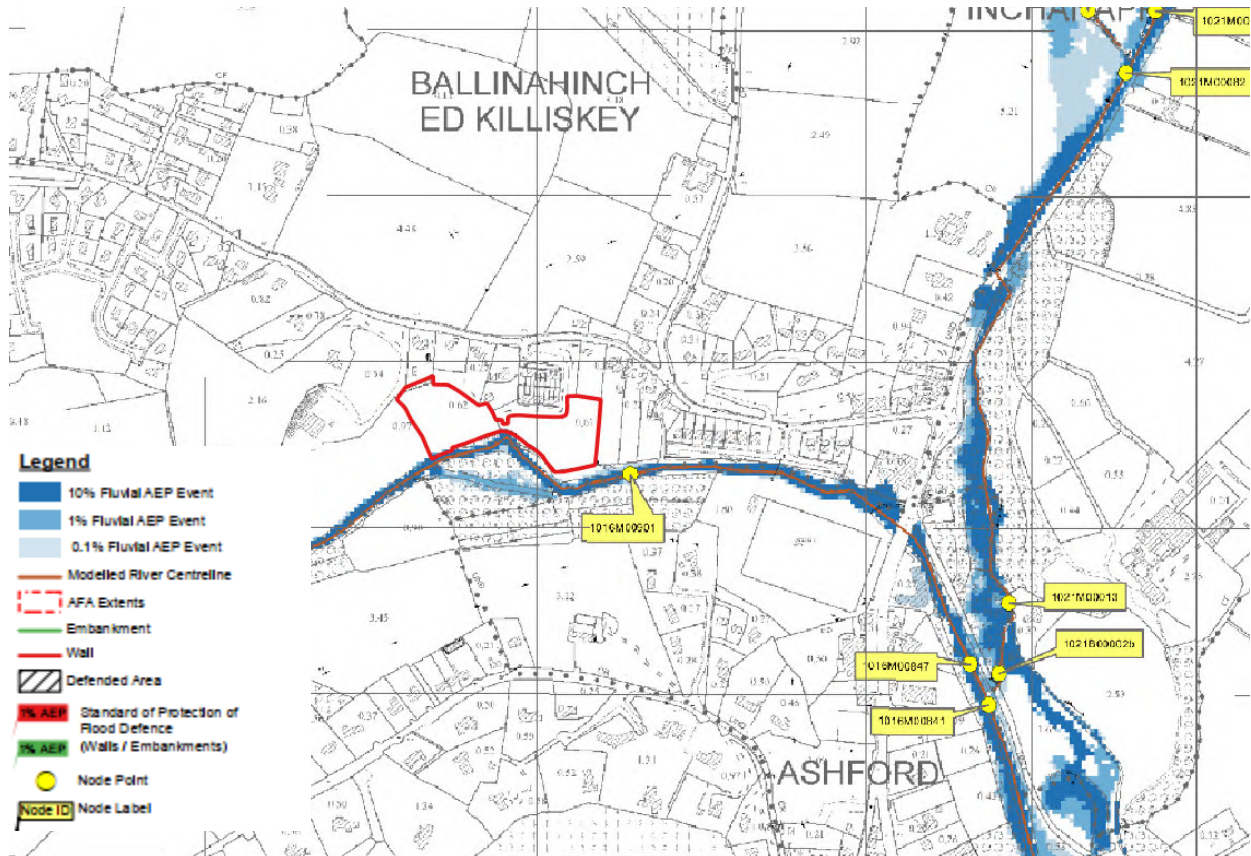
Figure 3-2: Extract from Eastern CFRAMS Final flood mapping
