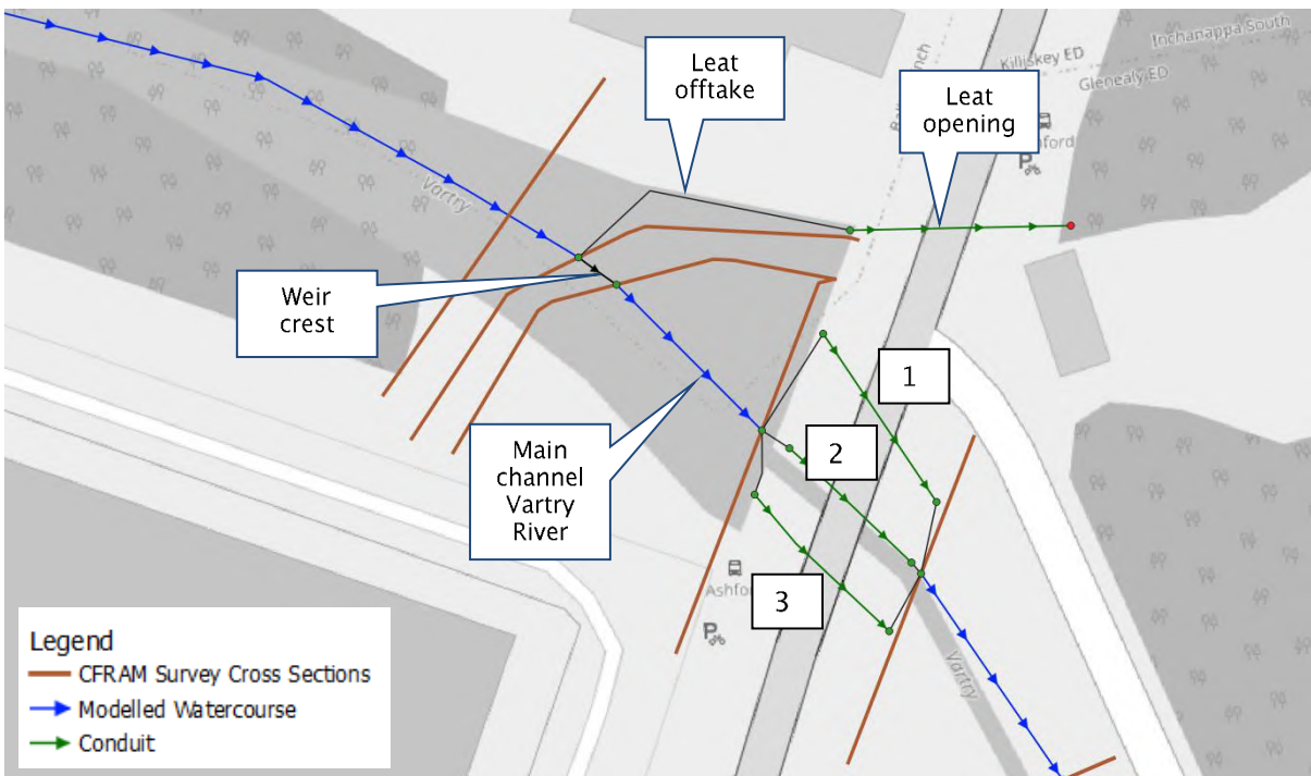
Figure 4-4: Modelled Structures
