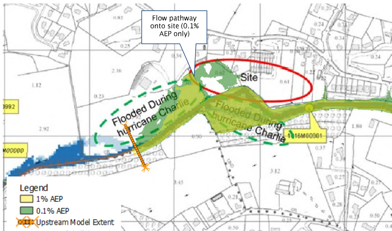
Figure 4-14: Modelled Vs Observed flood records
