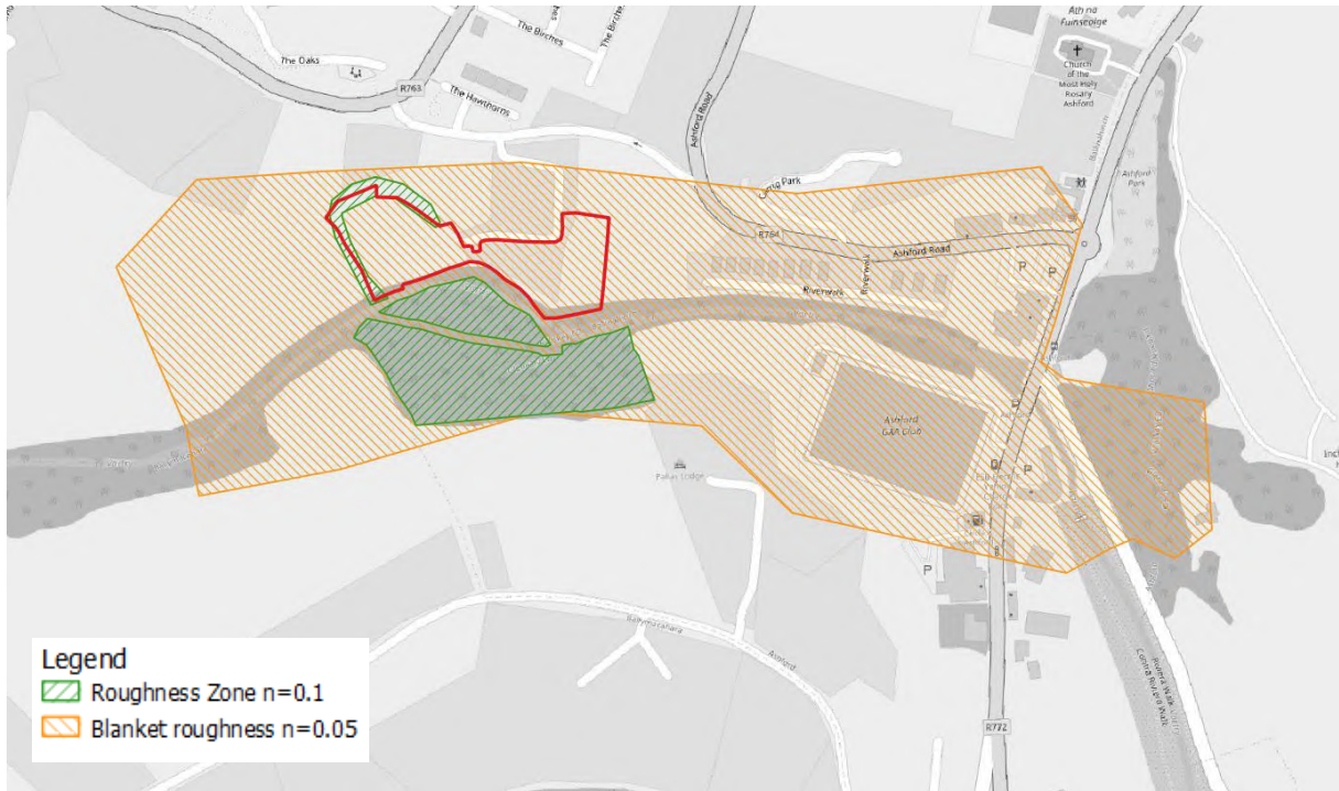
Figure 4-7: Roughness applied in 2D
