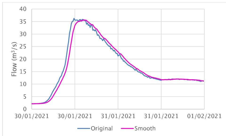
Figure 4-13: Largest observed flow hydrograph at Mount Ushers gauge: original vs smooth
